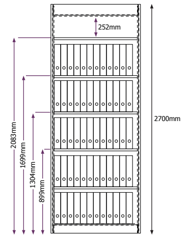
FOOLSCAP BOXFILE 368mm high x 75mm wide x 265mm deep
