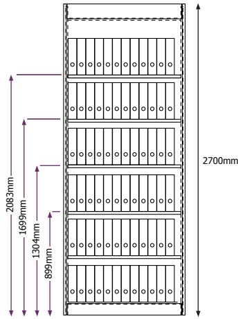
A4 LEVERARCH 318mm high x 75mm wide x 280mm deep
