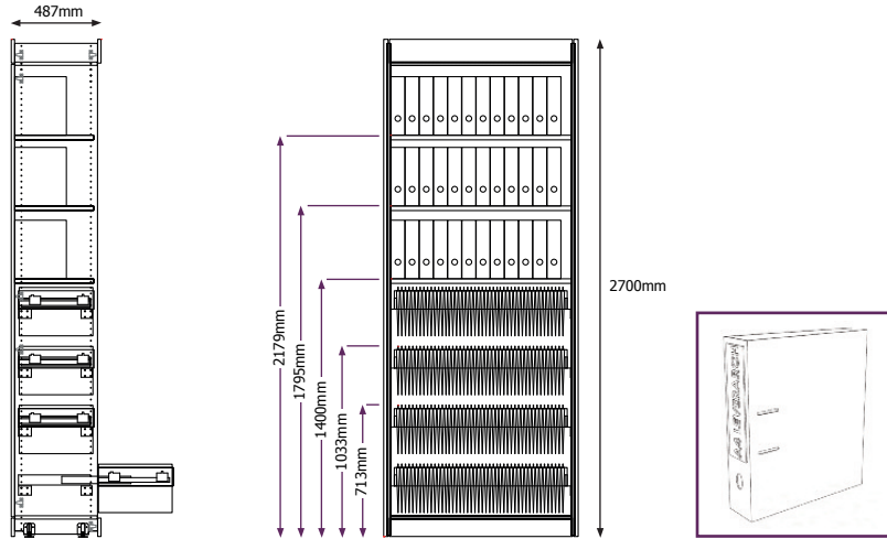
A4 LEVERARCH 318mm high x 75mm wide x 280mm deep
