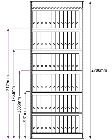
A4 BOXFILE 337mm high x 75mm wide x 265mm deep
